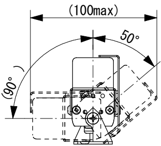
Adjustable Bracket
