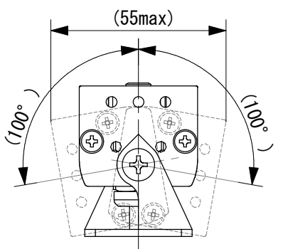
Adjustable Bracket (Not to Scale)
