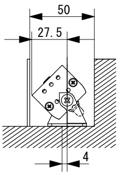
Adjustable Bracket (Not to Scale)
